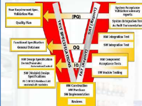
The GAMP 'V' Model V - MODEL for Specifications, Build and Testing
